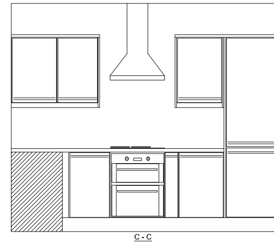
ELEVATIONS SCALE 1:20
