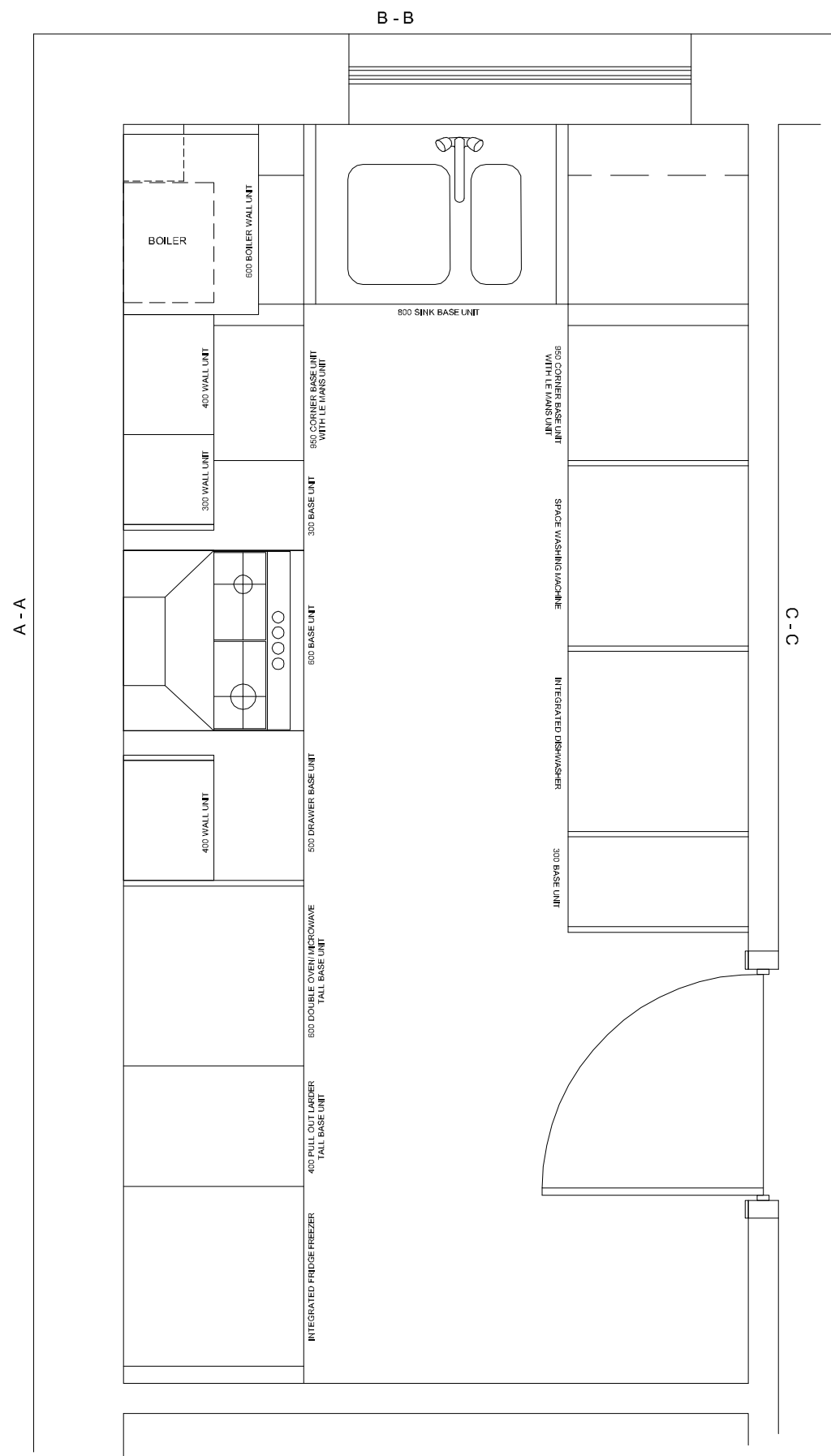
PLAN SCALE 1:10
