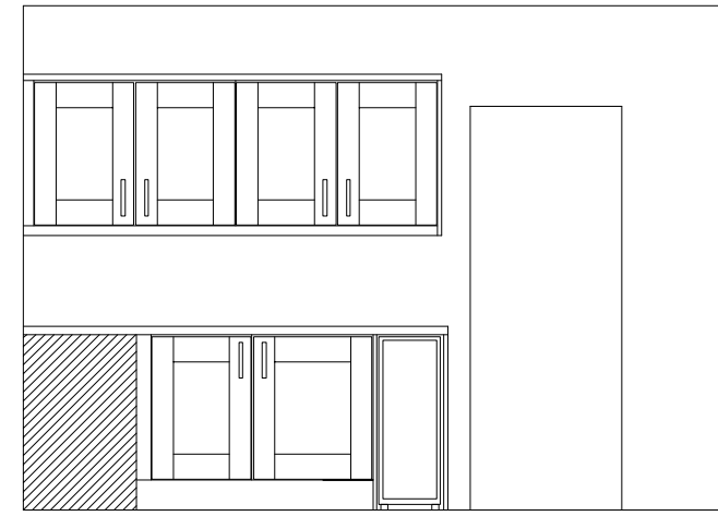
ELEVATIONS SCALE 1:20
