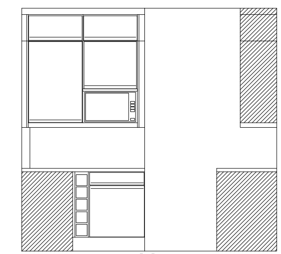
ELEVATIONS SCALE 1:20
