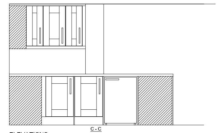
ELEVATIONS SCALE 1:20
