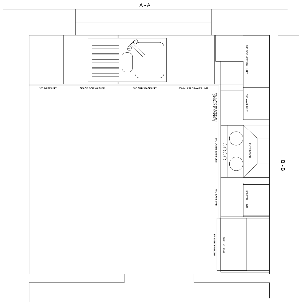
PLAN SCALE 1:10
