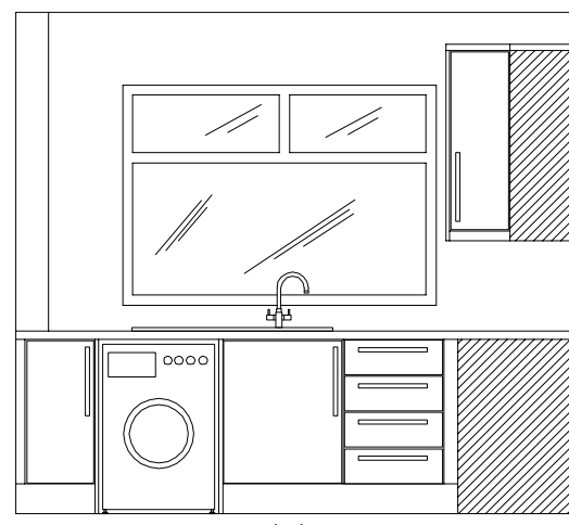
ELEVATIONS SCALE 1:20
